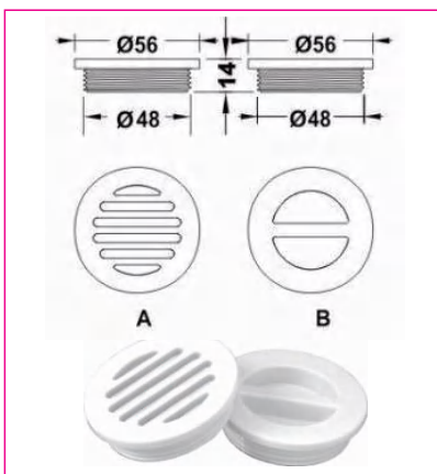
BW2022A/B 真空吸污配件面盖 Covers for suction fitting
