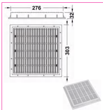
BW1032 方形主水器 Main drain cover
